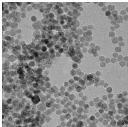
羧基化四氧化三铁纳米颗粒(7nm)的 TEM 图 TEM image of DMSA Coated Fe 3 O 4 Nanoparticles (7nm)
