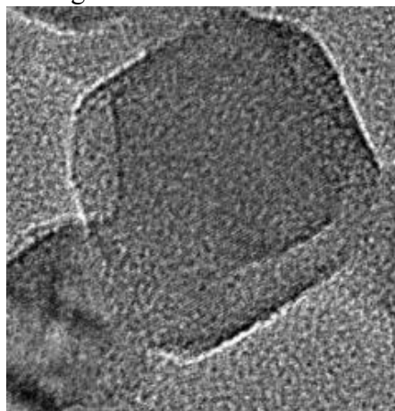
富勒烯 C60 的 TEM 图片 (50nm) TEM images of Fullerene C60 (50nm)
